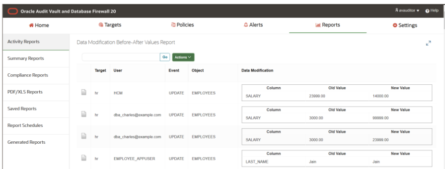
Figure 8. Data modification Before-After Values report in AVDF
