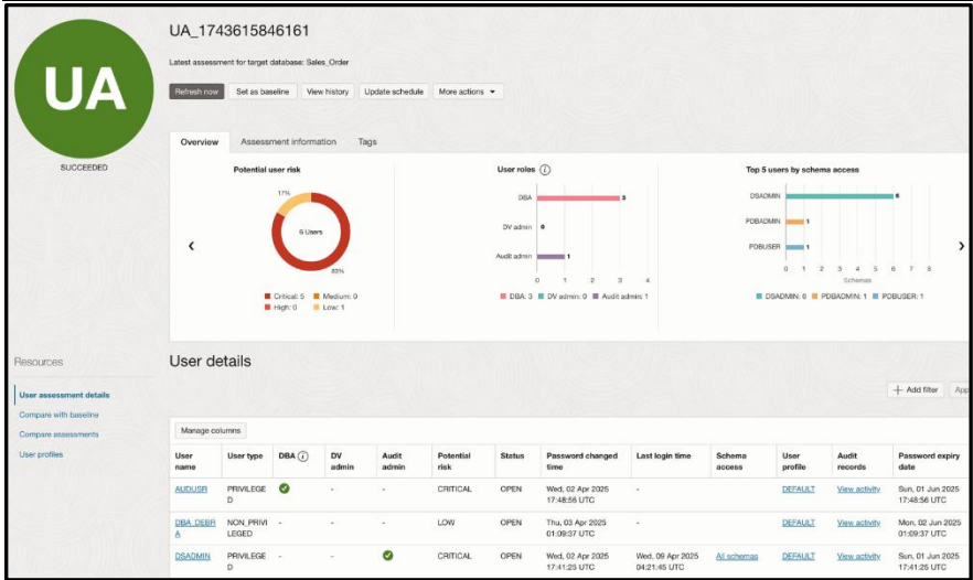
Figure 2. User Assessment report in Data Safe showing privileged users
