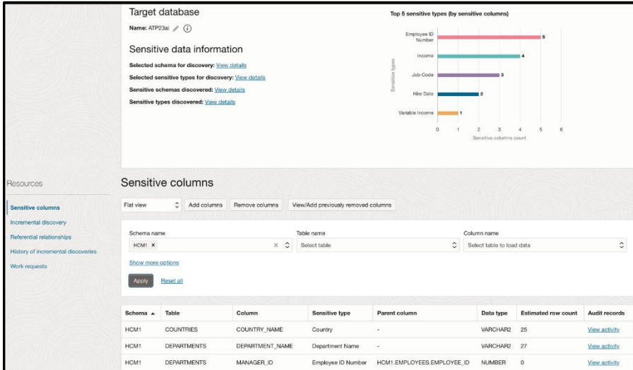
Figure 6. Sensitive data discovery feature in Data Safe
